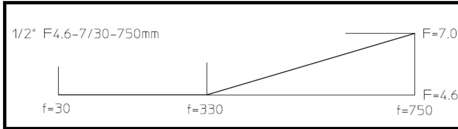
LMZ750 / LMZ750-XD F-Number Curve
