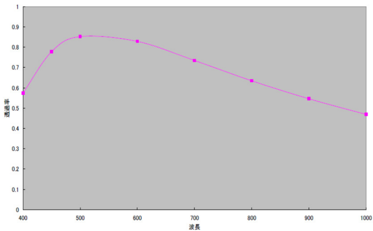
LMVZ3510A-IR Transmission Chart
