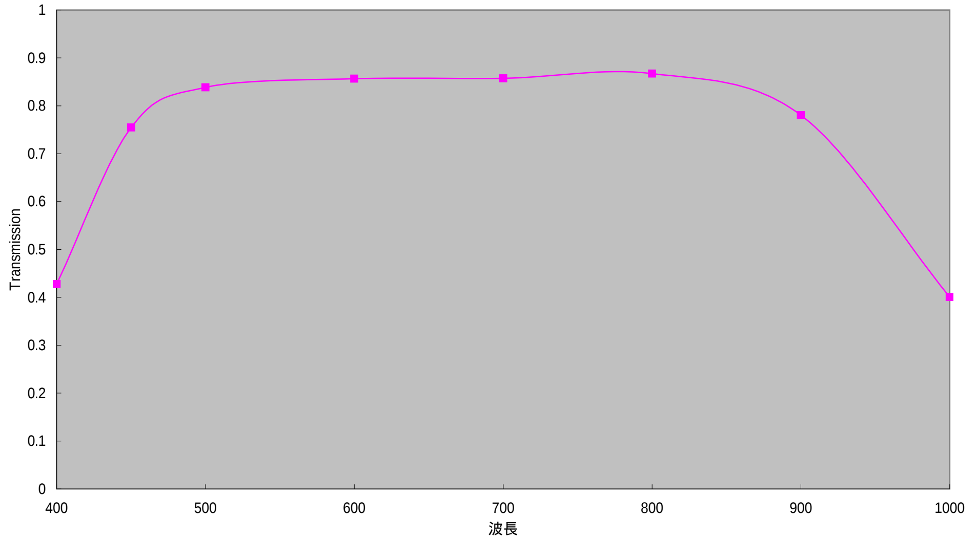
LMZ1236AMPDC-XD (1022) Transmission
