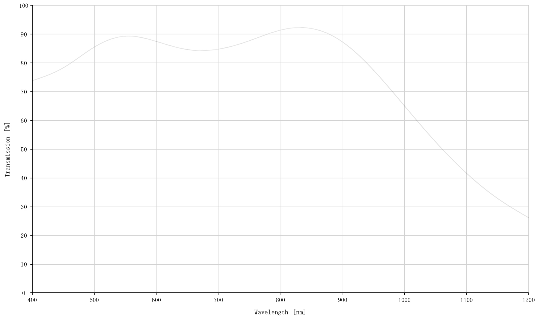
LM35VM Transmission
