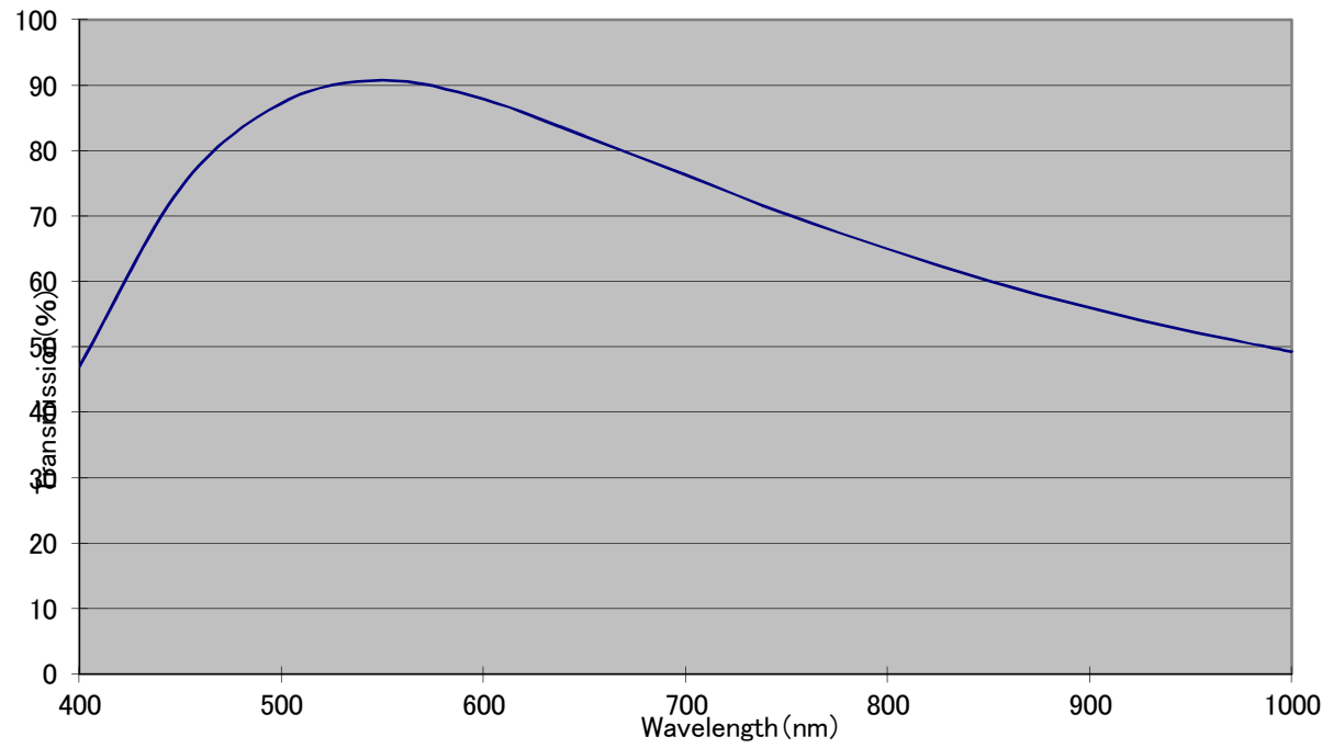
LM3NCM Transmission
