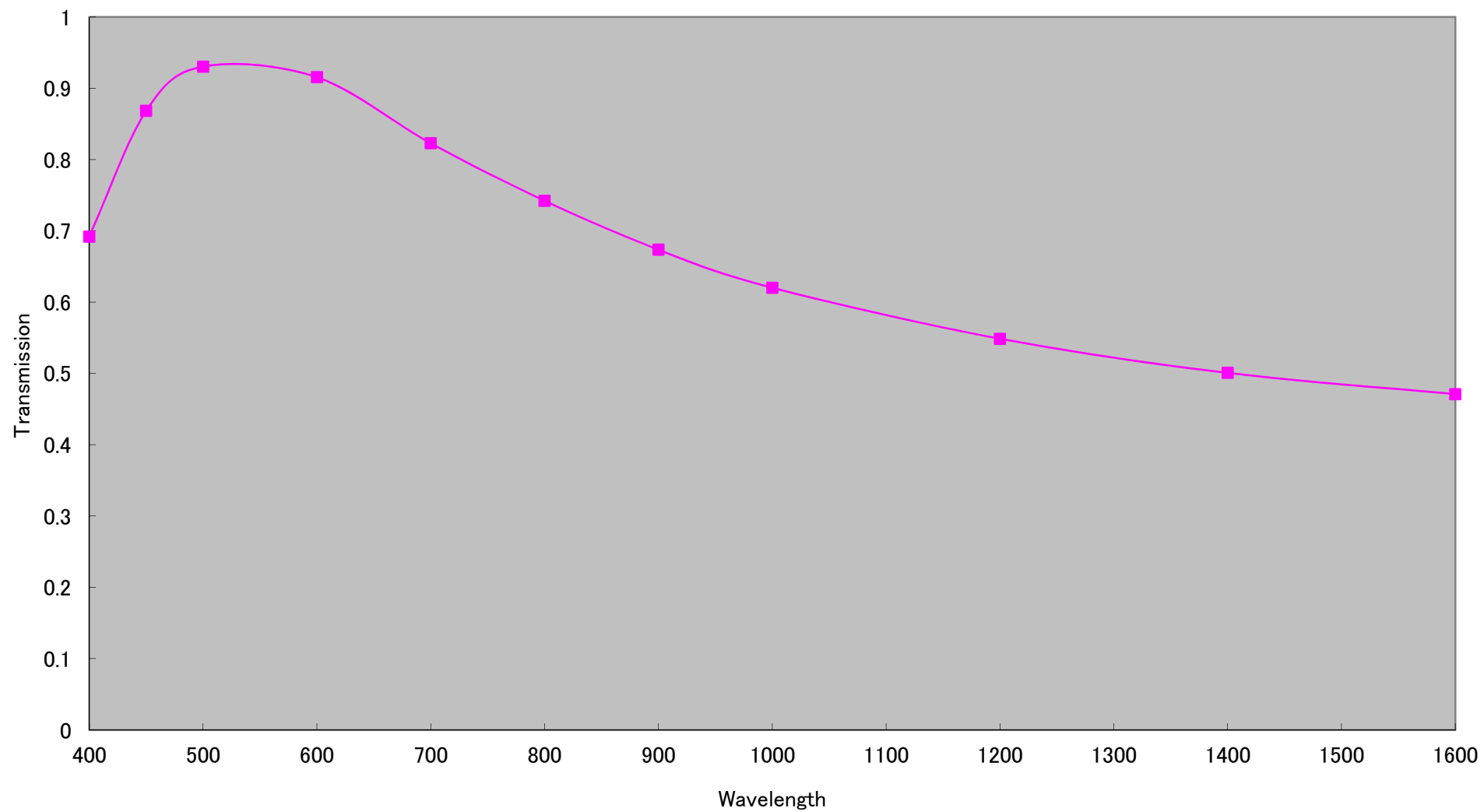
LM3NF (1033) Transmission
