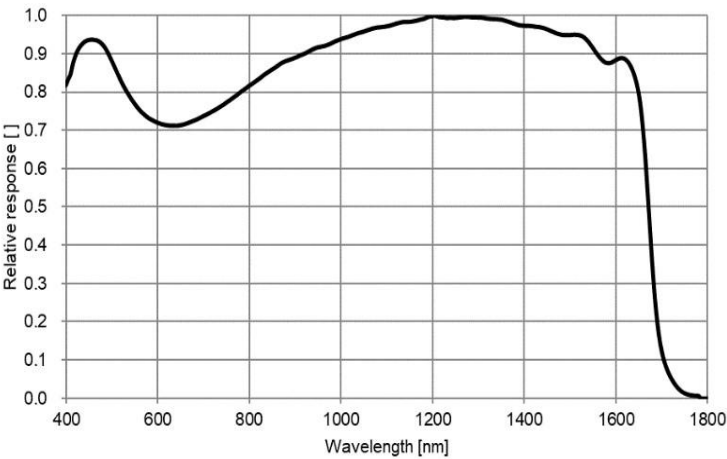
SWIR relative quantum efficiency
