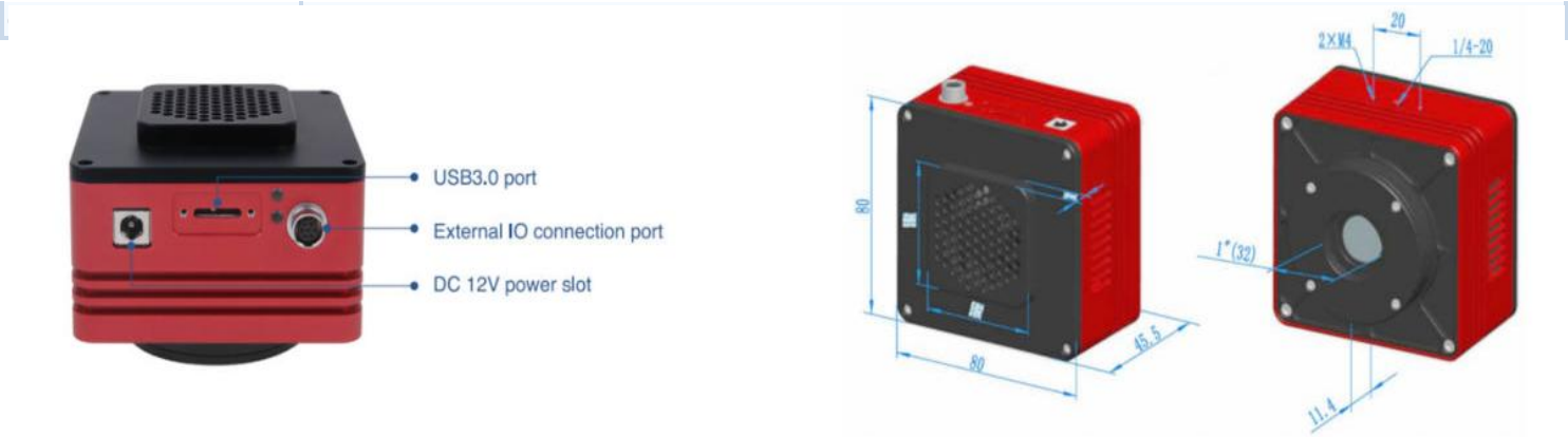
Camera Dimensions
